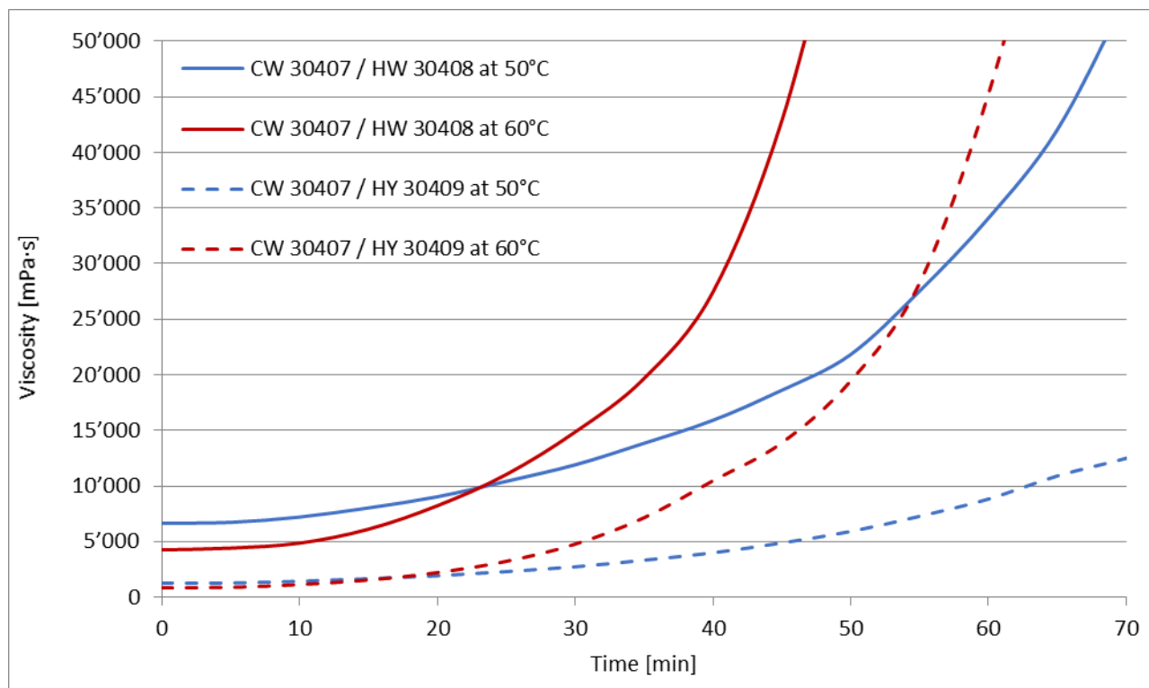
Fig.1 Viscosity increase at 50°C and 60°C (Rheomat 300 MS DIN 125 D= 10s-1)
