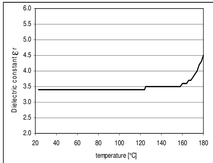
Figure 5: Rel. permittivity (ε r ) at 50 Hz (IEC 60250)
